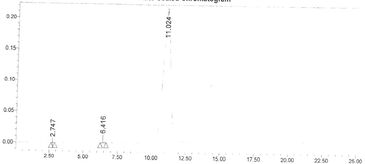
Peak Results
